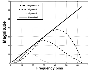
Figure 2: The response of the ideal differentiator and the first derivative of a Gaussian with standard deviation \sigma = 0.5, 1 and 2 .
