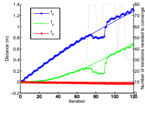
Figure 5: Estimation of the robot's translation (MPT_FC)
