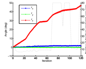
Figure 9: Estimation of the robot's rotation (MPT_ESM)
