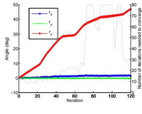
Figure 8: Estimation of the robot's rotation (MPT_FC)
