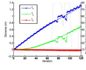
Figure 6: Estimation of the robot's translation (MPT_ESM)
